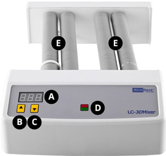
LC-3DMixer front
